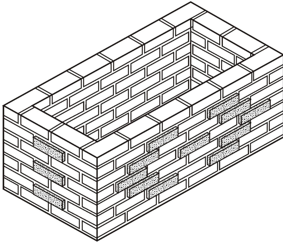
Hollow Pier Pictorial View
