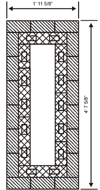
Section B - B
